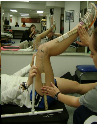
Figure 4: Active ROM
