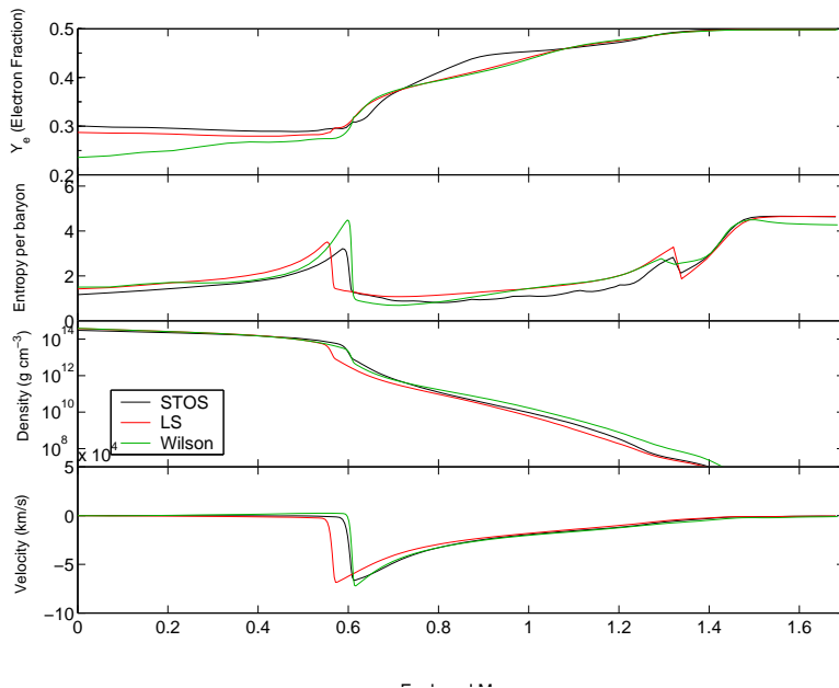
Figure 4.2: Bounce with the Bruenn85 rates
