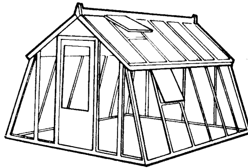
Figure 10. Slant leg.
