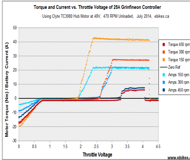
Figure 3: Relationship between driver throttle voltage and motor torque/battery current. [1]
