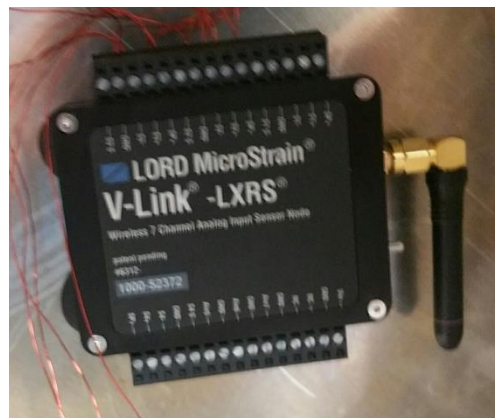
Figure 9: Wireless Node by LORD MicroStrain
