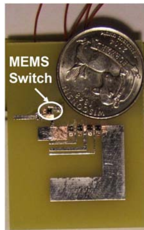
(b) Mini-nested reconfigurable patch
