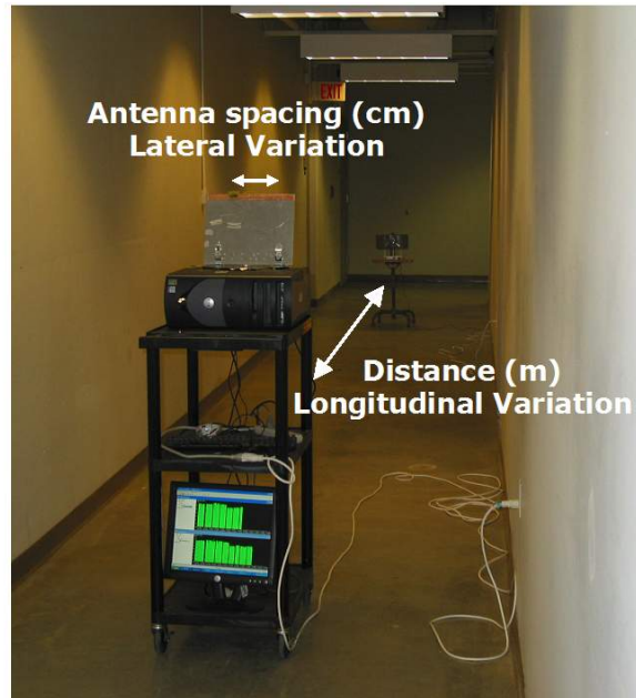
Figure 4.20. Measurement setup in a corridor scenario. The longitudinal distance between Tx and Rx varies from 24~80 \lambda and lateral variation between single band PIFA is 0~0.8 \lambda .
