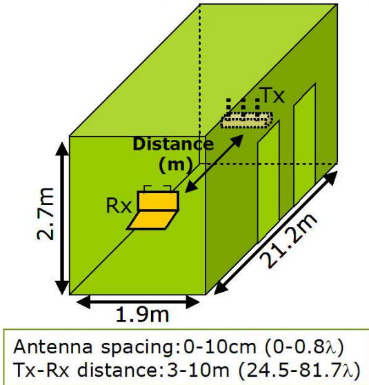
Figure 4.20. Measurement setup in a corridor scenario. The longitudinal distance between Tx and Rx varies from 24~80 \lambda and lateral variation between single band PIFA is 0~0.8 \lambda .
