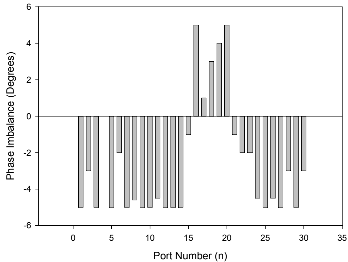
Figure 2.12. Radial Combiner transmission coefficient S_{1n} phase variations, where phase ( S_{1n} ) was measured between port 1 (center port) and port n ( n is any peripheral port where n = 2, 3, \dots, 30 ) while all other ports are match-terminated. The above figure shows the phase deviation of the transmission coefficient for all peripheral ports. The measured phase imbalance is within \pm 5 degrees above average.
