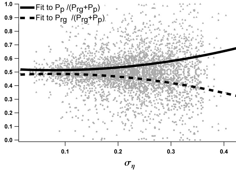
Figure 4.6: Given the efficiencies, the proposed distribution outperforms the ratio-Gaussian distribution, on average, as asymmetries in the efficiencies increase, as measured by the efficiency standard deviation \sigma_\eta .
