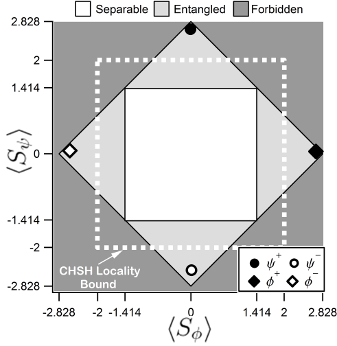
Figure 2.10: Separable and entangled state bounds for parameters \mathcal{S}_\psi and \mathcal{S}_\phi with corresponding measurement values for the four prepared Bell states indicated by dots and diamonds.
