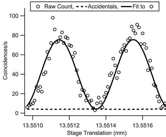
Figure 2.2: Non-Local Franson Interference for detectors HA0 and HB1 with 99.6 \pm 2.6\% corrected visibility and a 89.5 \pm 2.3\% raw visibility. This date was collected using a preliminary Mach-Zehnder experiment.
