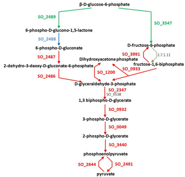
Shewanella oneidensis MR-1: superpathway of glycolysis and Entner-Doudoroff
