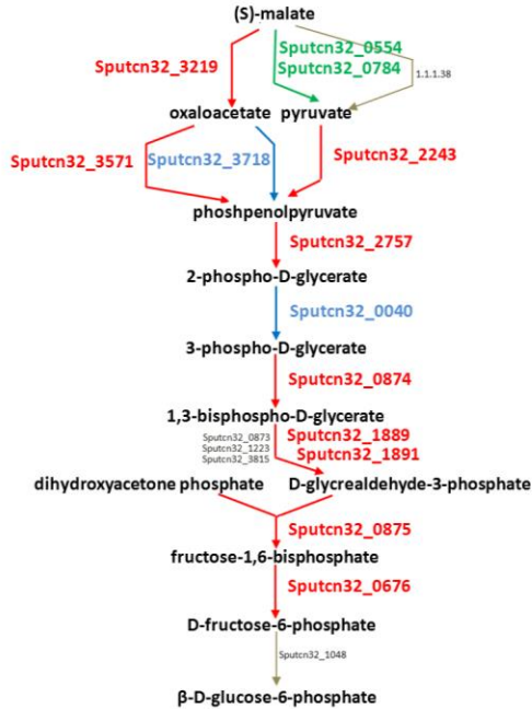
Shewanella putrefaciens CN-32: gluconeogenesis I pathway
