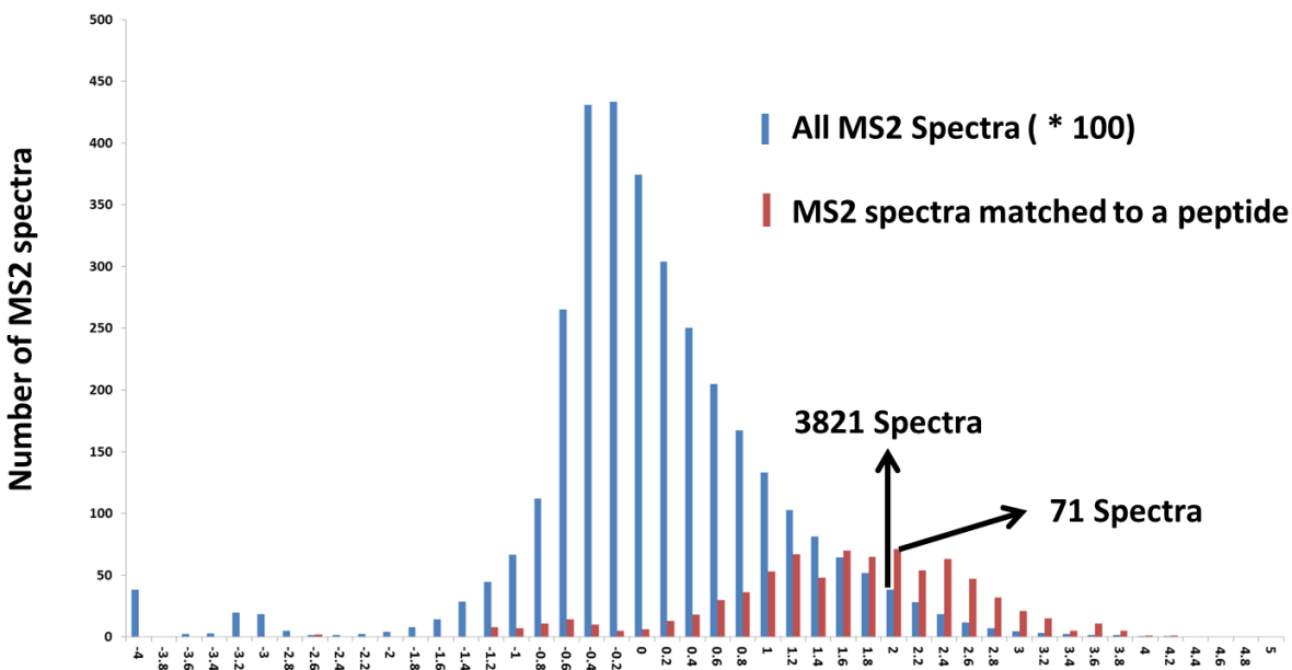
Figure 4.3 Plot of ScanRanker score with respect to the total number of MS/MS scans acquired from Sample 10 . The red bars represent the total number of experimentally identified scans (1 unique peptide, 5% Q-value) for Sample 10 by MyriMatch database searching against F14TB database (~7.8 million sequences)
