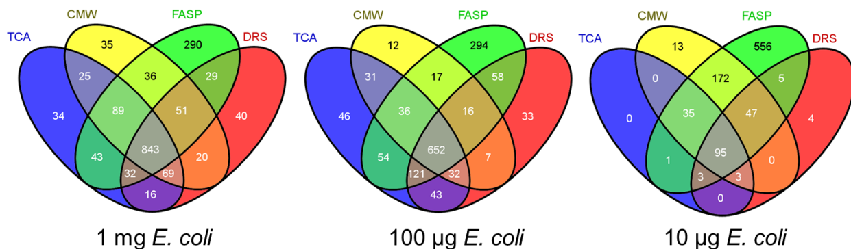
Figure 3.3 Unique and common proteins identified in E. coli K-12 lysate after SDS lysis / removal using four different methods and three different protein amounts
