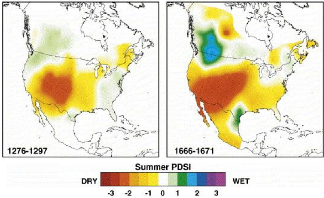
Figure 2.4: Tree-ring reconstructed summer PDSI during two multi-year droughts centered over the Puebloan cultural area. Similar to the Middle Cumberland, depopulation occurred in the American Southwest during drought periods (reproduced from Cook et al. 2007).
