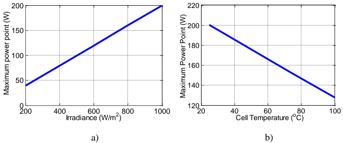
Figure 14. Relationship of KC200GT panel Maximum Power Point (MPP) with a) irradiance; b) Cell Temperature.
