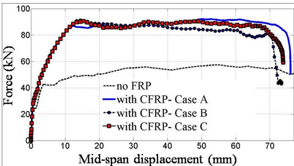
Figure 16. The behaviour of the beam with 40% degree of corrosion using different corrosion variants
