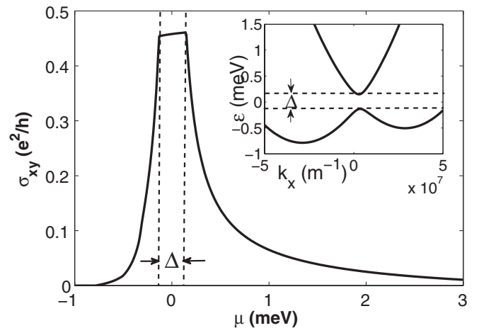
FIG. 2. Anomalous Hall conductivity versus chemical potential \mu at zero temperature for a two-dimensional electron-doped semiconductor. We have used \alpha_R = \alpha_D = 4.74 \times 10^4 m/s, m^* = .067m_e , and h_y = 0.2 meV. The electronic band structure versus k_x is shown in the inset along with the minimum energy gap \Delta indicated by the dashed lines.
