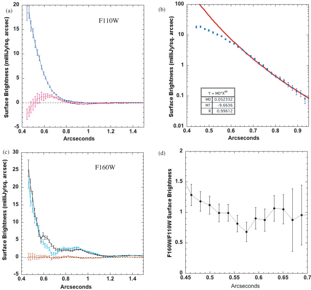
Figure 8. Disk azimuthally median SB: (a) F110W, from the first visit, and residuals from a PSF–PSF subtraction handled similarly to the SAO 206462 data. The disk is a 14\sigma detection near the coronagraph’s inner working angle. (b) Power-law fit. (c) SB for F160W. PSF subtraction results for the single science target orientation are shown with each PSF template, together with a red PSF–PSF pair. (d) The F160W/F110W radial SB ratio of the disk. While a shallow color gradient is seen for r \lesssim 0''.59 , overall the disk is significantly blue compared to the star ( f_{F160W}/f_{F110W} = 2.27 \pm 0.60 ). Error bars in panels a–c are the standard deviations of SB measures (and ratios in panel d) from all unmasked pixels in concentric 1 pixel (75.8 mas) wide annuli (radially incremented in 1/4 pixel-wide steps) about the corresponding annular medians. The 1\sigma measurement errors do not include a systematic \lesssim 20\% uncertainty in the absolute calibration of the SB due to the uncertainties in the flux-density renormalization (brightness scaling) of the PSF templates before image subtraction.
