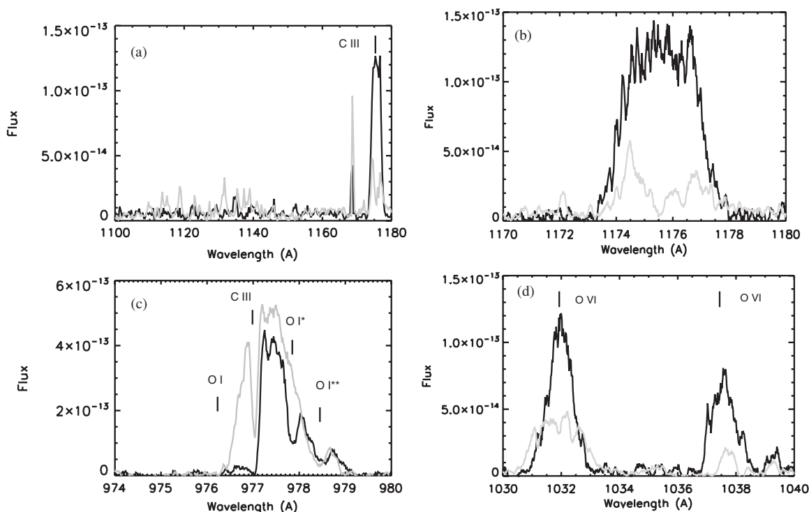
Figure 4. FUV data for SAO 206462 (black), and comparison stars HD 139614 and MWC 480. (a) A faint continuum is present in the spectra of MWC 480 (gray) and SAO 206462 from 1090 to 1180 Å. (b) The C III \lambda 1176 profile for SAO 206462 has the blocky shape characteristic of chromospheric emission profiles rather than the double-peaked emission seen in MWC 480 (gray). (c) The C III \lambda 977 profile, while chopped up by O I absorption has a type I P Cygni profile indicating the presence of a high velocity, moderate temperature wind similar to that observed by Dupree et al. (2005) in TW Hya. This wind is not seen in HD 139614 (gray). (d) The O VI profile for SAO 206462 is narrow compared to MWC 480 (gray) which is typical of the jet-driving Herbig Ae stars, but is broad compared to moderate v \sin i transition region sources.
