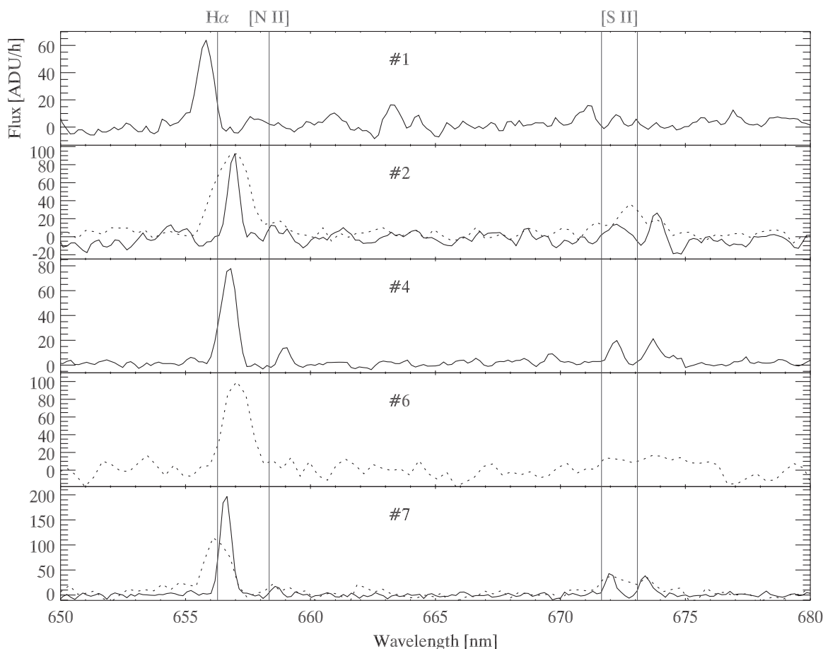
Figure 8. Spectra of the HH 728 knots detected in the Tautenburg Schmidt data, with the same numbering as in Figure 7. Dashed spectra are from 2002, taken with a 2" slit and R \sim 500 , while the solid line spectra are from 2006, taken with a 1" slit at R = 2000 . HH728-1 is clearly blueshifted, while the other knots are redshifted.
