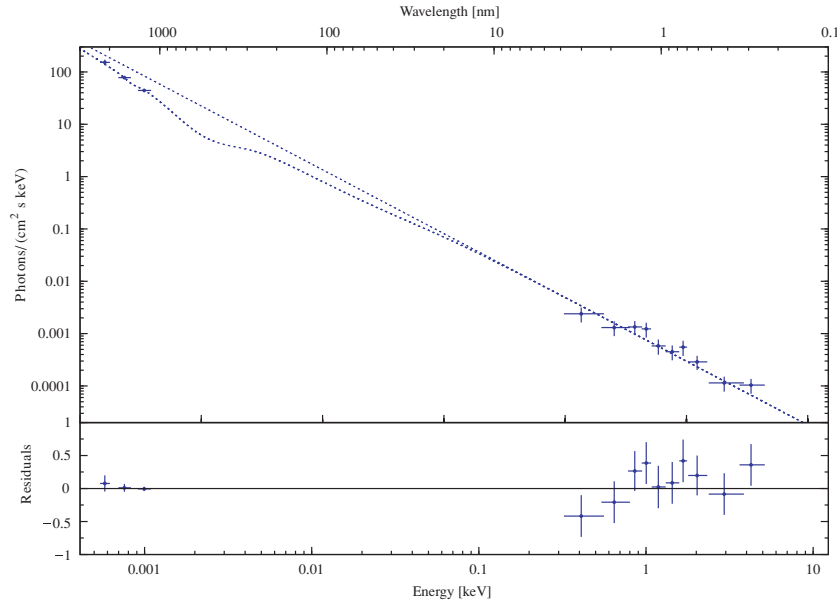
Figure 5. Combined Swift /XRT and GROND SED for the time interval 200–1800 s after the burst. Shown is the fit with a single power law (for parameters, see the text).
