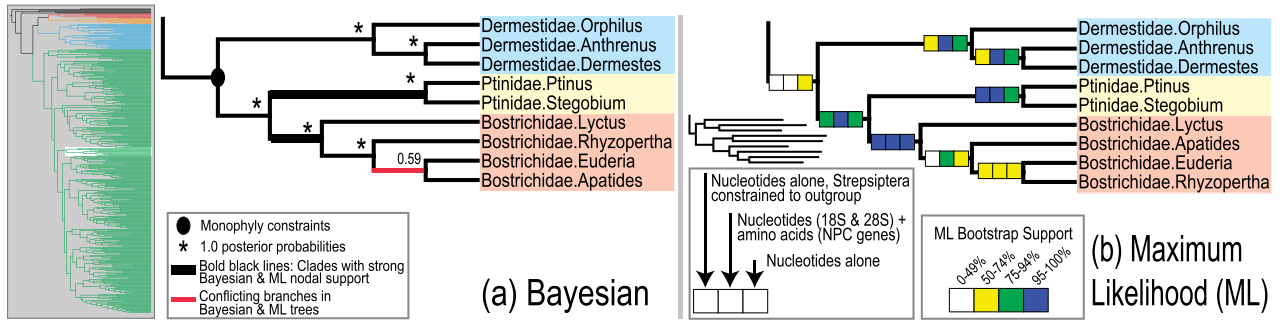
Fig. 10. (a) Bayesian and (b) maximum-likelihood (ML) summary trees for Bostrichoidea resulting from partitioned phylogenetic analyses of DNA sequences from eight nuclear genes (see Materials and methods). We included data from all extant families of Bostrichoidea except Endecatomiidae. However, we did include Endecatonus (Endecatomiidae) in preliminary analyses (not shown here; see Discussion). Statistical measures of Bayesian posterior probability (BPP) support are shown along branches in the Bayesian tree (an asterisk indicates nodes with maximal BPP support of 1.0). Partitioned ML bootstrap support under various analytical schemes is noted by coloured boxes along branches in the ML tree (see embedded legends). Background colours indicate major clades present in both trees. Monophyly constraints from the BEAST analysis are shown as black ovals (see Table S3).
