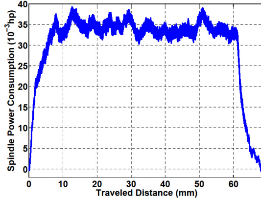
Figure 4: Cutting power for Test 1.3
