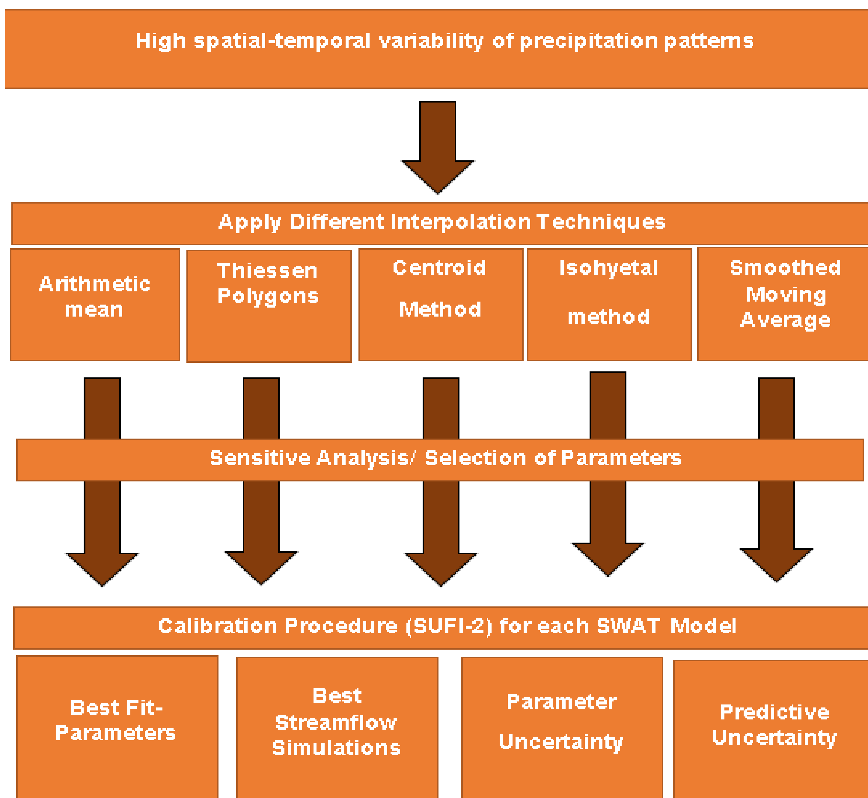
Figure 2: Methodology Flowchart
