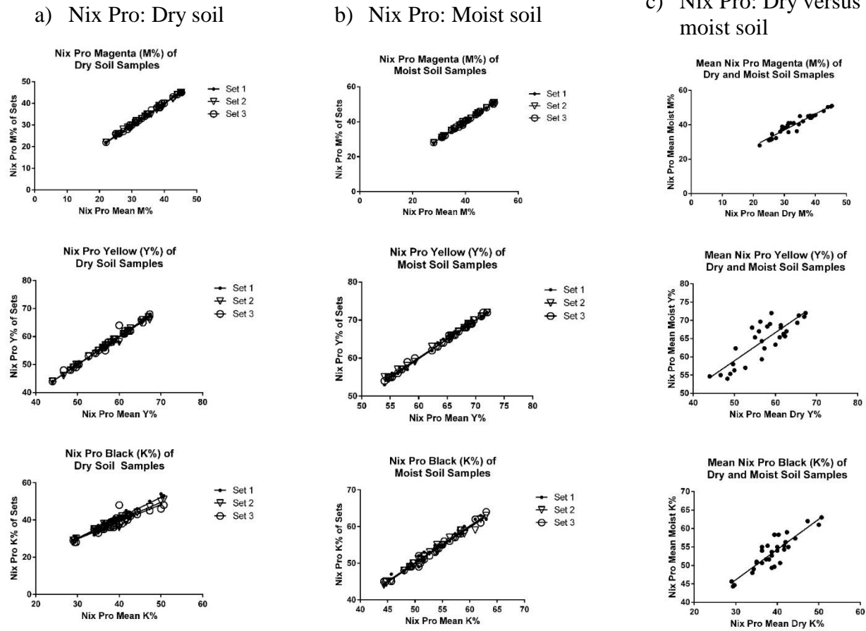
Fig. 2. Nix Pro Color Sensor CMYK color code means vs. Nix Pro Color Sensor CMYK scan sets in dry and moist soil and mean CMYK color codes in dry vs. moist soil ( n = 31 soil samples for each set, corresponding correlation ( r -value) and significance ( p -value) data are reported in Tables 2 and 3).
