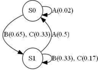
Figure 4.3: HMM of the inter-packet Delays Inside VPN
