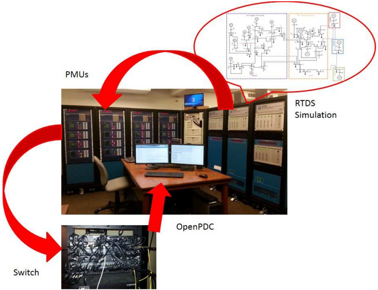
Figure 3.1: Laboratory Setup
