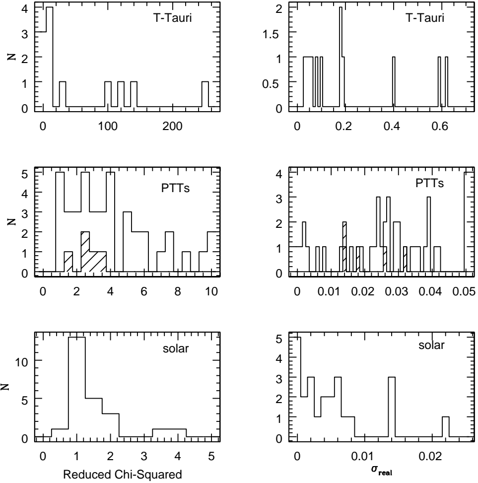
Figure A.8 Histograms for \chi^2_\nu and real dispersions ( \sigma_{real} ) for HIPPARCOS V-magnitude variability. We have presented them in order of theoretically decreasing variability from the top down (i.e. TTs have the highest amount of irregular variability and solar analogs the lowest). The post T Tauri plot includes the 5 candidates we identify (shaded histogram) and a sample of 41 post T Tauri stars identified from the literature (unshaded histogram).
