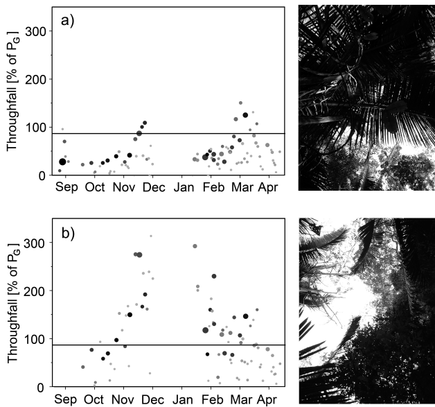
Fig. 3. Temporal patterns of throughfall percentages of incident rainfall for two collectors standing only 5 m apart from each other. Each event is represented by a dot whose diameter is proportional to rainfall amount. Varying colours from light grey to black illustrate low and high rainfall intensity ( I_{10 \text{ max}} ) values, respectively. The photographs on the right site show the vegetation above these two collectors.
