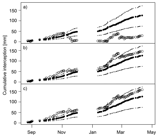
Fig. 4. Cumulative totals of calculated (open circles) and estimated (solid circles) interception for (a) all collectors ( n=20 ), (b) collectors not showing temporal patterns of throughfall percentages ( n=9 ) and for (c) collectors without obvious influence of the palm species Orbignya phalerata ( n=6 ). The dots indicate the uncertainty of the modeled interception resulting from the uncertainty in S_C .
