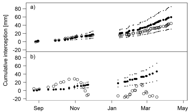
Fig. 6. Cumulative totals of calculated (open circles) and estimated (solid circles) interception for maximum 10 min rainfall intensities (a) I_{10\max} \leq 30 \text{ mm h}^{-1} and (b) I_{10\max} > 30 \text{ mm h}^{-1} including all collectors ( n=20 ). The dots indicate the uncertainty of the modeled interception resulting from the uncertainty in S_C .
