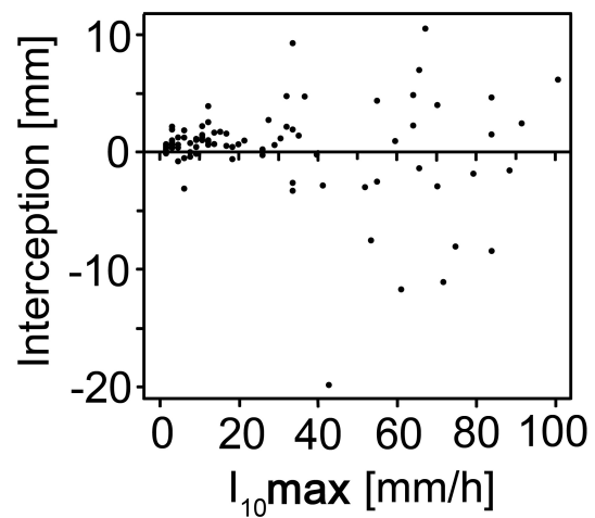
Fig. 5. The relationship between calculated interception and maximum 10 min rainfall intensity ( I_{10\text{max}} ).
