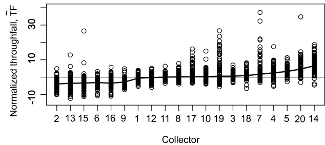
Fig. 2. Plot of normalized throughfall, \tilde{T} , for the whole period. Each circle represents the event throughfall volume at a single collector, normalized to zero median and unit variance for that event. The collectors are plotted on the horizontal axis and ranked by their means, \tilde{T} , which are connected by the black curve.
