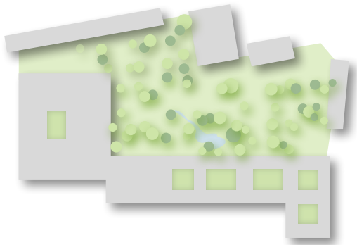
Figure 71: Perforated, articulated buildings with narrow building footprint to maximize daylighting and connections to nature, Hospital Basel, Switzerland.
