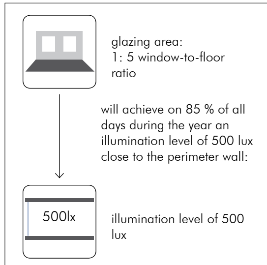
Figure 52: Size of glazing area and its relationship to interior illumination levels.
