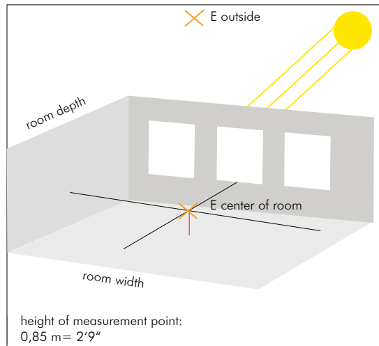
Figure 51: Calculation of daylight factor (DF).
