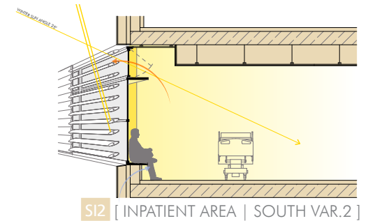
Figure 148: Shading concept for inpatient areas facing south.
