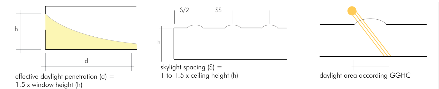
Figure 118: Effective daylight penetration, calculation of skylight spacing and qualification as daylight area according to GGHC.
