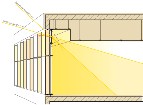
Figure 72: Vertical blinds for eastern/ western facade for non-inpatient area.
