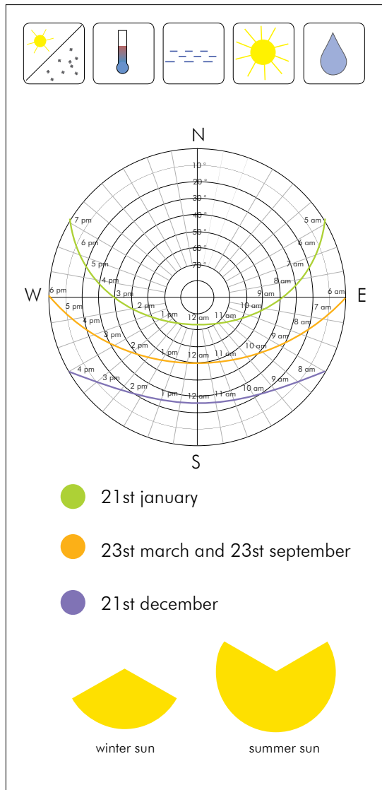
Figure 129: Climate characteristics and sun path chart for site in Norristown.
