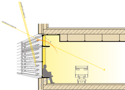
Figure 73: Horizontal blinds on southern facade for an inpatient area.
