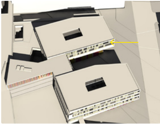
Figure 140: Daylight simulation: 23rd April, 9 am, patient rooms in upper inpatient tower receive direct morning sun. Only parts of the surgery and imaging are cast from shadow from lower inpatient unit pavilion.
