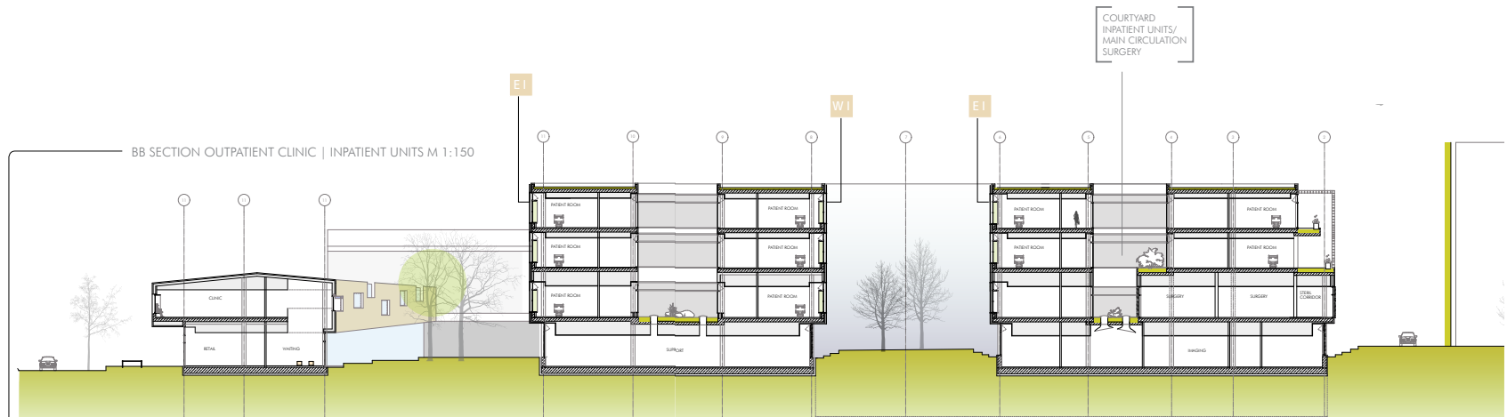
Figure 166: Section through inpatient pavilions and courtyard
