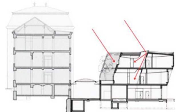
Figure 116: Section through inpatient unit, Knittelfeld Hospital, Austria
