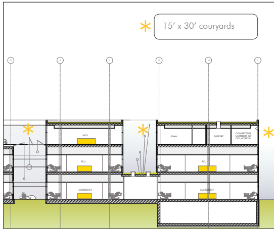
Figure 155: Section through diagnostic and treatment: emergency, PACU and NICU.
