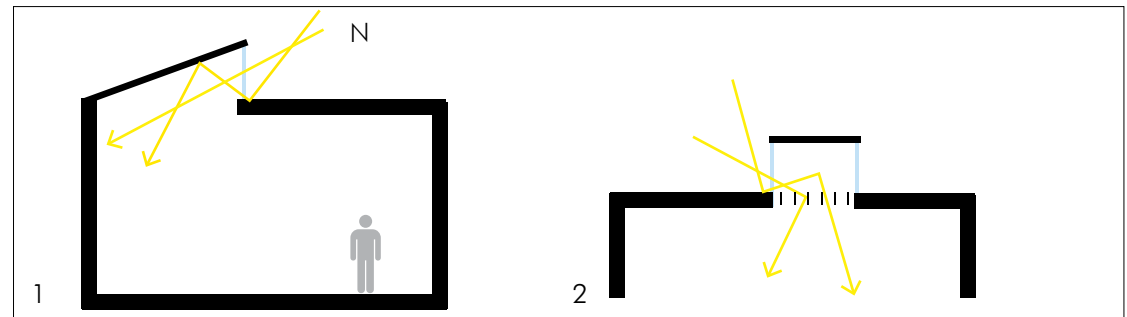
Figure 112: Sun control strategies diffuse daylight distribution: clerestory facing north (1) and clerestory with redirecting blinds (2).
