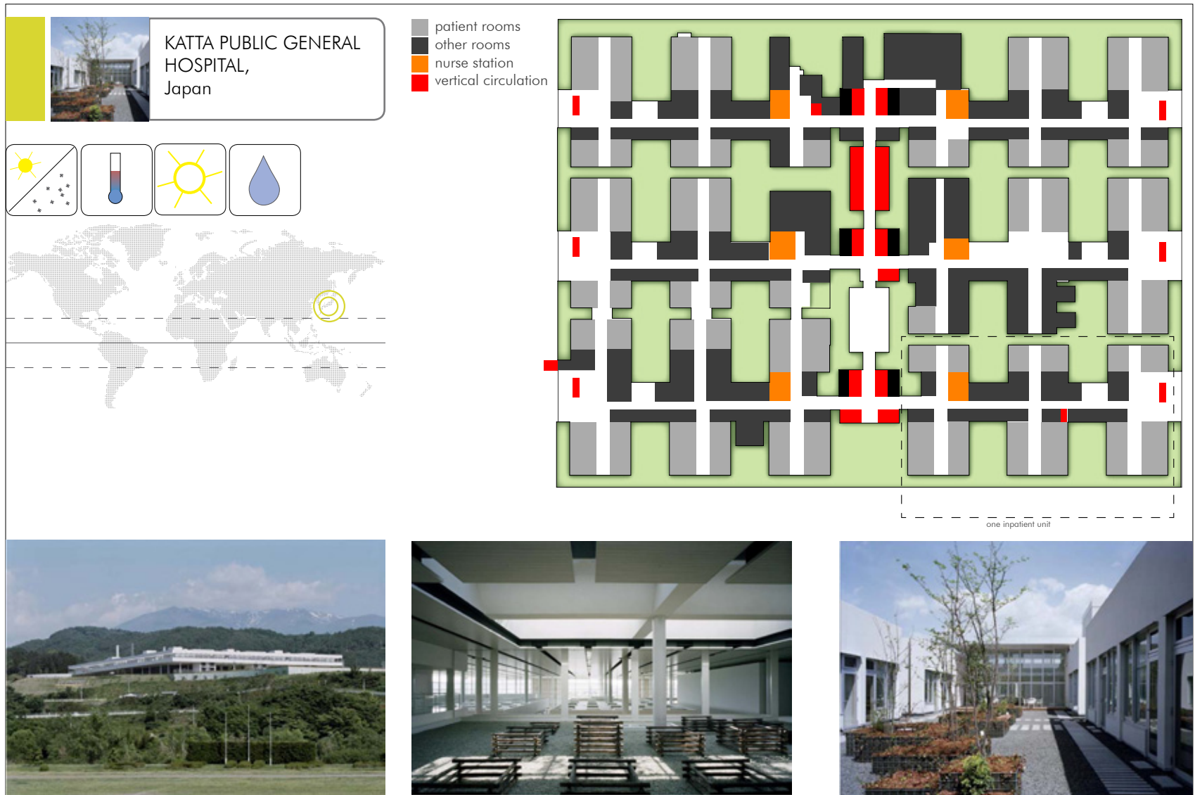
Figure 101: Spreadsheet, Katta Public General Hospital, Japan
