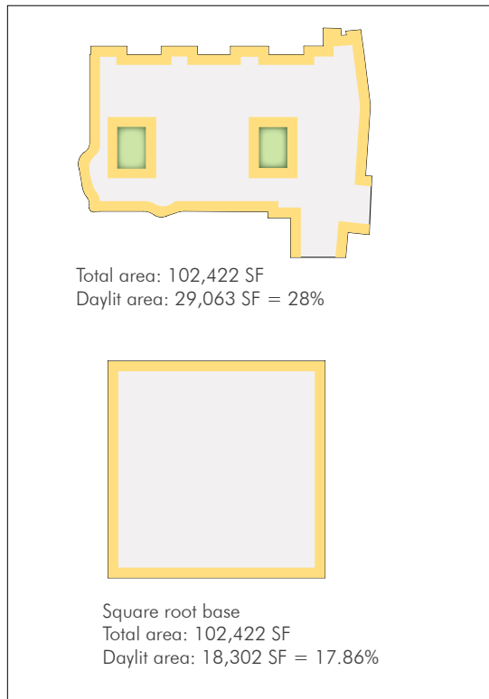
Figure 35: GGHC perimeter calculation for the diagnostic and treatment department of the Palomar Pomerado Health Medical Center, CA.
