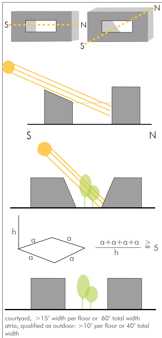
Figure 96: Courtyard design principles for optimized daylighting.
