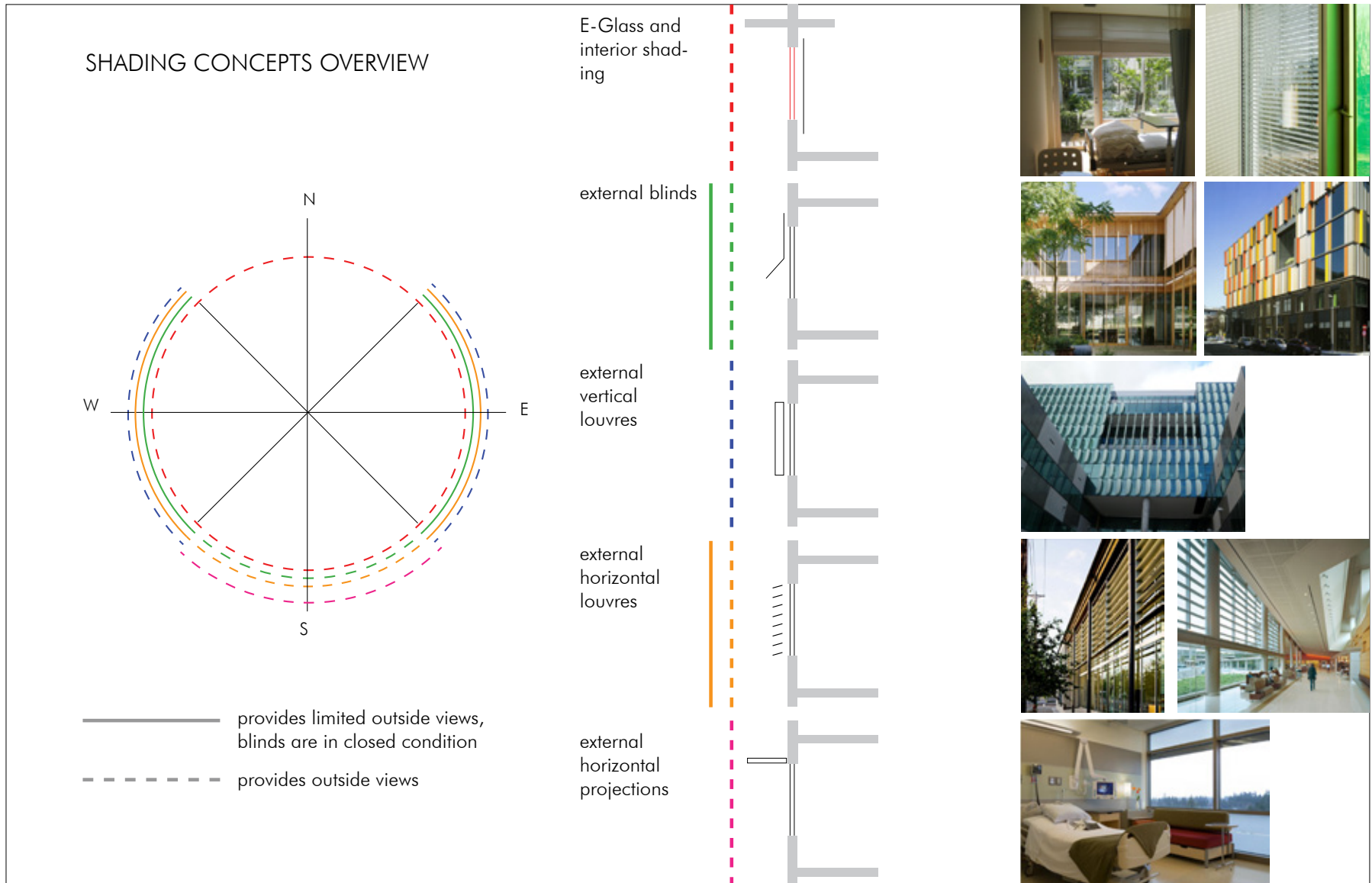
Figure 108: Spreadsheet illustrating different shading concepts for different directions.
