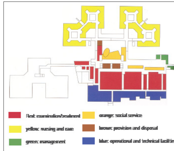
Figure 48: Departmental plan, Community Hospital Agatharied, Germany.
