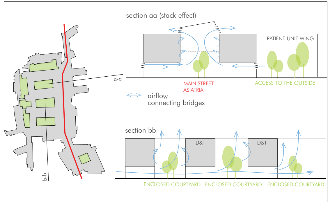
Figure 81: Natural ventilation principles, Rikshospitalet Oslo, Norway
