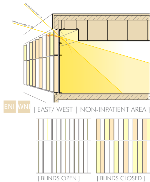
Figure 144: Shading concept for non-inpatient areas facing east or west.
