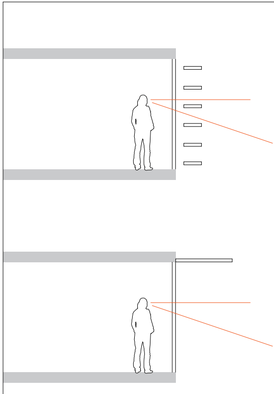
Figure 104: Sun control on southern facades.
