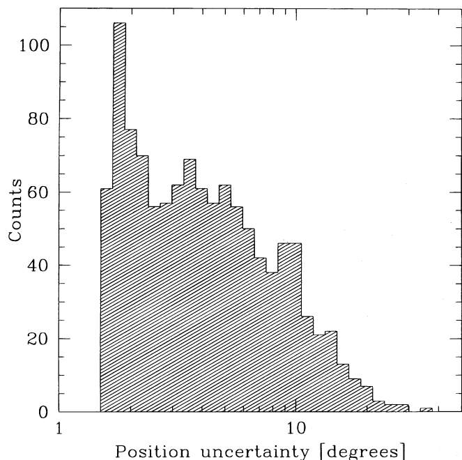
FIG. 2.—A histogram of the position errors \Delta\theta is shown for the BATSE 3B sample of 1122 gamma-ray bursts. The 1^{\circ}6 systematic errors are included here, added to the statistical errors in quadrature.
