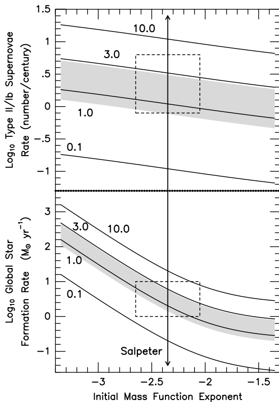
FIG. 1.—Global star formation rate (lower panel) and current Galactic Type II + Ib supernova rate (upper panel) vs. the IMF exponent. Each labeled curve corresponds to a different Galactic ^{26}\text{Al} mass (in solar masses), with the preferred ^{26}\text{Al} mass range (0.7–2.8 M_{\odot} ) imposed by the COMPTEL observations shown as the gray bands. The horizontal dimension of the dashed boxes are centered on a Salpeter -2.35 exponent and are representative of the range of IMF exponents for massive stars encountered in the literature. Vertical dimensions of the dashed boxes were set by requiring consistency between the COMPTEL estimates of the Galactic ^{26}\text{Al} mass and the simple model for the ^{26}\text{Al} injection rate from massive stars. This consistency then appears to imply a Galactic SFR during the past million years of 5 \pm 4 M_{\odot} \text{ yr}^{-1} , and a core-collapse supernovae rate of 3.4 \pm 2.8 per century.
