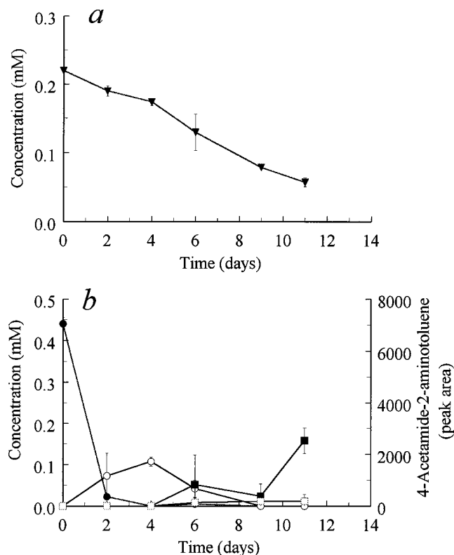
FIG. 5. Biotransformation of 2Am4NT (a) and 4Am2NT (b) by P. aeruginosa . Error bars indicate 1 standard deviation of duplicate samples. Symbols: ▼, 2Am4NT; ●, 4Am2NT; ○, 4Ac2m2NT; ■, 4-acetamide-2-aminotoluene; □, DAT.
