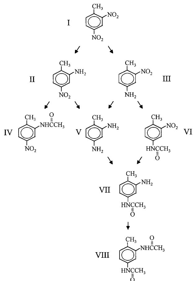
FIG. 6. Proposed pathway for the reduction and acetylation of DNT by P. aeruginosa . I, DNT; II, 2Am4NT; III, 4Am2NT; IV, 2Ac4AmNT; V, DAT; VI, 4Ac2AmNT; VII, 4-acetamido-2-aminotoluene; VIII, 2,4-diacetamidetoluene.
