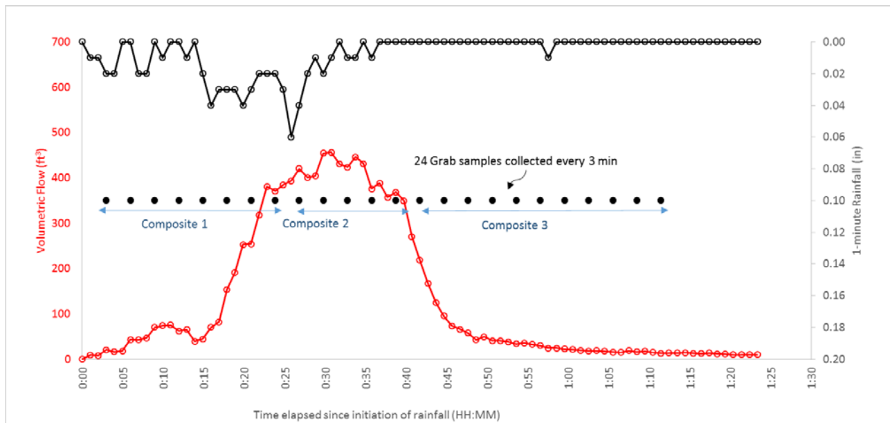
Figure 1. Storm hydrograph collected at 1st Ave S, NMB on 7/10/2014 22:58 to 7/11/2014 0:32 LST. Total rainfall accumulation: 0.63 inches. Total discharge: 11041 cubic feet.
