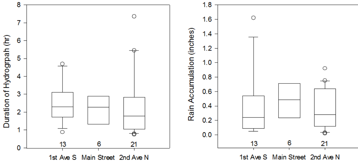
Figure 2. Box plots showing preliminary hydrograph duration (left) and rain accumulation (right) at the three pre-construction sampling sites in NMB, SC
