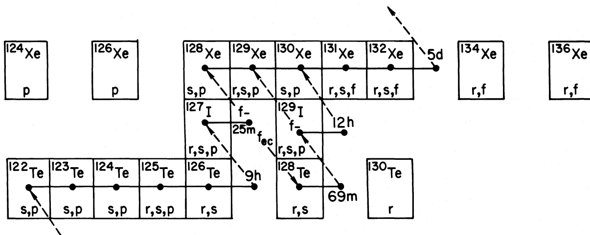
FIG. 1.—The s -process neutron-capture chain through Te, I, and Xe is shown by solid line connecting the points. The dashed lines indicate weak decays; for example, f_- ( ^{128}\text{I} ) is the fraction of 25m ^{128}\text{I} that undergoes negatron emission during the s -process. The dominant contributing processes to nucleosynthesis of each isotope are designated by p , s , r , f in order of yield.
