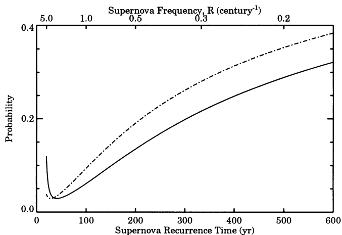
FIG. 5.—The total probability that the mean supernova rate equals or exceeds the value shown, given the SMM 1.16 MeV measurement. The calculation assumes Poisson-distributed events and considers only the flux from the latest event, which is assumed to have occurred at distance 8.5 kpc. The ^{44}\text{Ti} production per event is a function of the rate, M_{44} = 3.6/R , such that the inferred production rate of ^{44}\text{Ca} today is maintained. The solid line assumes that the ^{44}\text{Ti} half-life is 67 yr ( \tau_{44} = 0.96 ), the dot-dash line, 46 yr ( \tau_{44} = 0.67 ).
