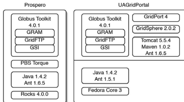
Fig. 7. Prospero and UAGridPortal software stacks
