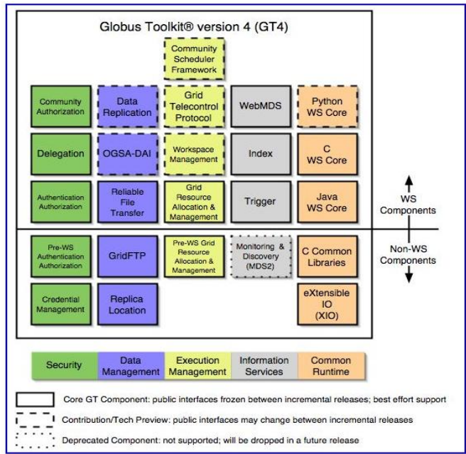
Fig. 2. Globus Toolkit Version 4 architecture [20]
