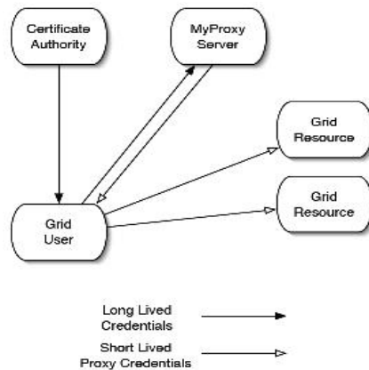
Fig. 5. Credential Management with a MyProxy server
