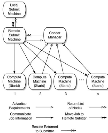
Fig. 4. Condor-C job handling
