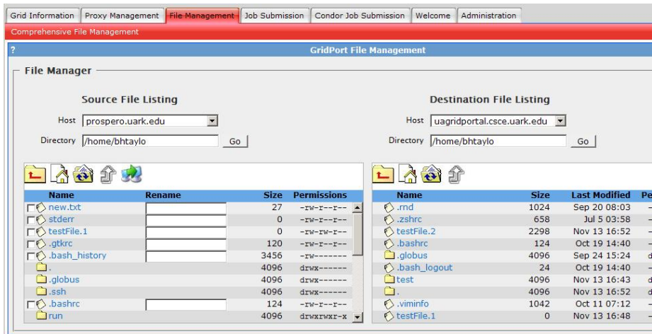
Fig. 11. GridPort File Management Portlet
