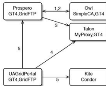
Fig. 6. User interaction with security components of the UA Grid
