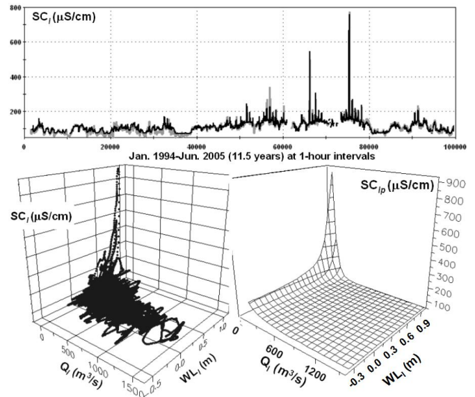
Figure 3. Modeling Savannah River Estuary seawater intrusion. Lower left – three dimensional scatter plot of specific conductance (SC) versus with freshwater flow ( Q ) and sea water level ( WL ). Above - measured (gray) and ANN-predicted (black) SC. Lower right - ANN response surface fitted to scatter plot data.
