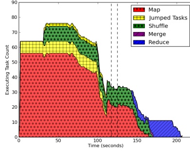
(b) Jump during map phase of wordcount execution
