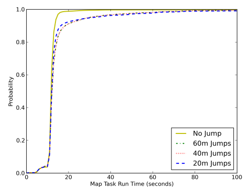
(b) Terasort Map Task Run Time CDF
