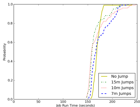
(a) Wordcount Job Run Time CDF
