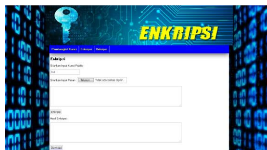
Gambar 12 Interface Enkripsi
