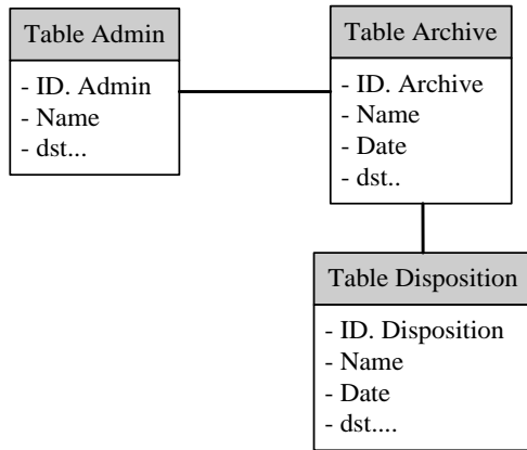
Fig. 6 Relationship Table
