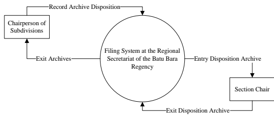
Fig. 2 Diagram Context
