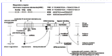
Figure 7. Molecular model of the gene regulation of retinoic acid (RA) action (George Zhu, January 1991, revised in 2012). Schematic alignment of the receptor protein. The two highly conserved regions, identified as the putative DNA-binding (C) and hormone-binding (E), a hinge region (D) and the non-conserved variable NH 2 -terminus (A/B) as described above. CAT:CAAT box, CCAAT-enhancer binding proteins (or C/EBPs); GC:GC box; TATA:TATA box. (Figure from Zhu G, Curr Pharm Biotechnol, 2013, 41(9):849-858) [20,207]
