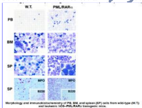
Figure 4 shows pml/RAR \alpha fusion in differentiation block at promyelocytic stage in transgenic mice (Figure from He LZ, et al, Proc Natl Acad Sci USA, 1997, 94:5302-07) [166]
