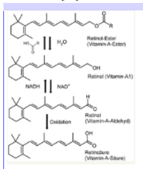
Figure 1. Chemical structure of retinol,one of the major forms of Vitamin A
