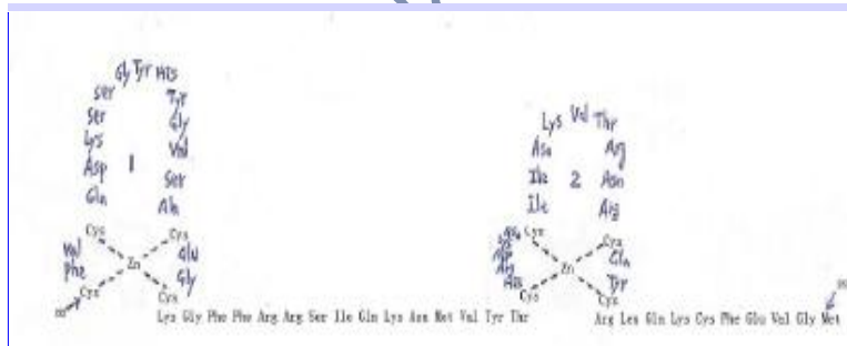
Figure 2. Amino acid sequence of the DNA binding domain of the hRAR \alpha into two putative zinc-binding finger (Figure from George Zhu a feeling for scientific drawing based on Evans RM,Science,1988,240:899-895; Beato M,Cell,1989, 56: 335-344; Giguere V,Nature,1987;330:624-29; Petkovich M, Nature, 1987,330: 444-450)
