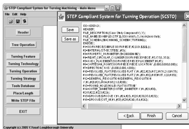
Fig 6 The SCSTO prototype
