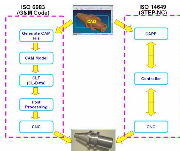
Fig. 1 Comparison of the CAD/CAPP/CAM process chain with ISO 6983 and ISO 14649
