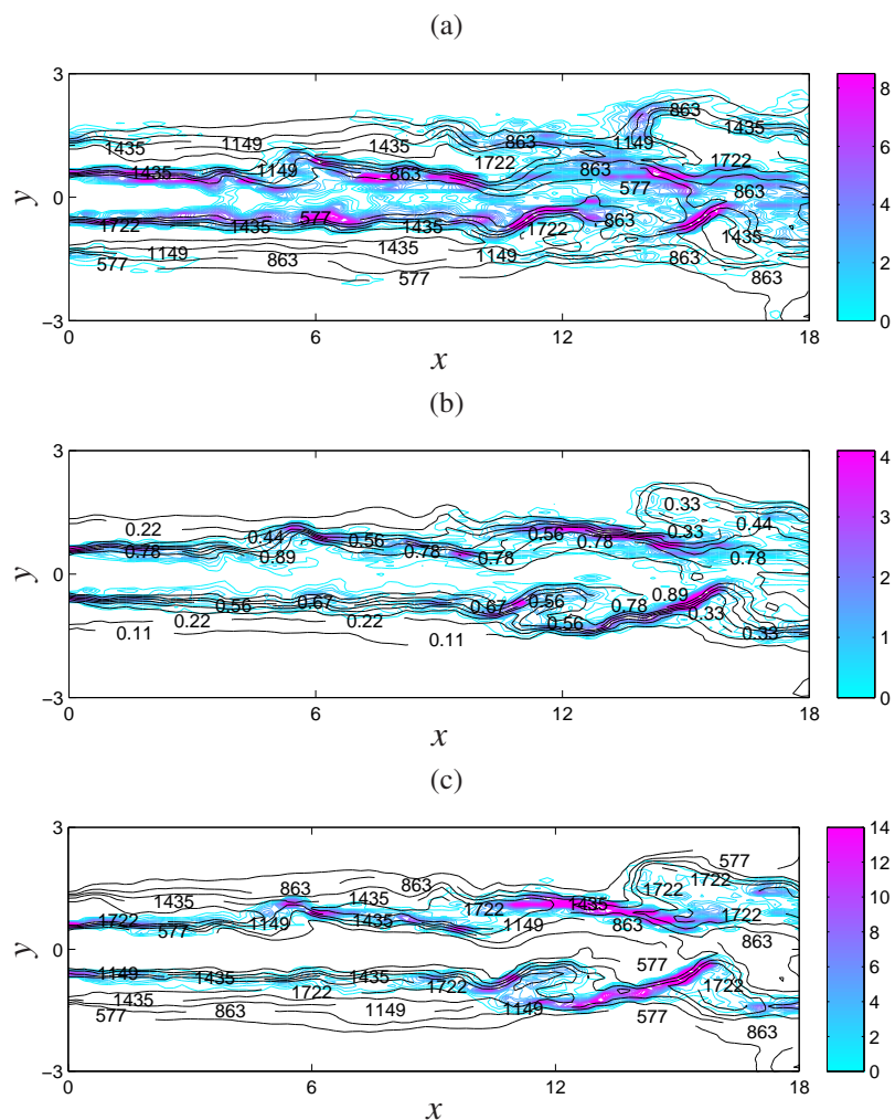
Figure 8. Instantaneous contours of entropy generation terms in Sandia Flame D simulations: (a) heat conduction (color) with temperature [K] (black) contours, (b) mass diffusion (color) with mixture fraction (black) contours and (c) chemical reaction (color) with temperature [K] (black) contours.
