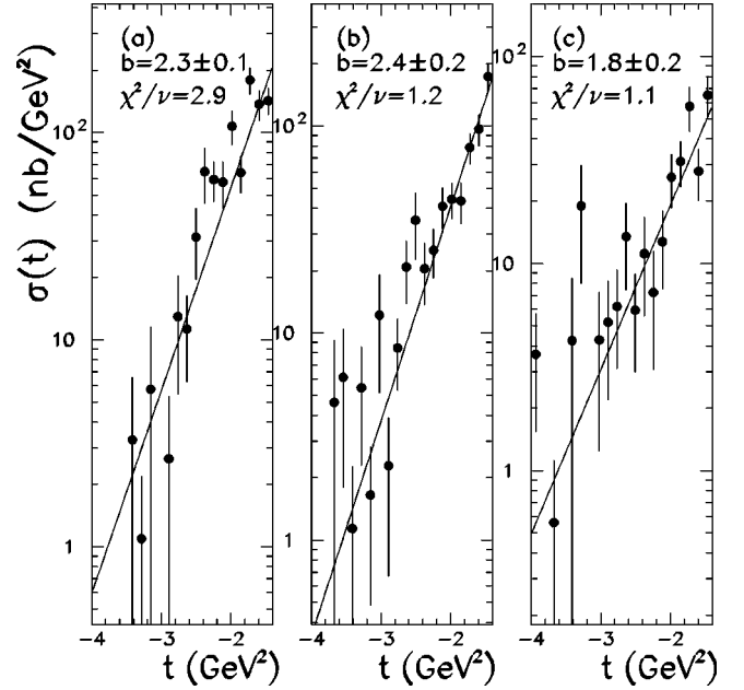
FIG. 6. The t distributions for three regions of W : (a) 1.95 < W < 2.21 GeV, (b) 2.21 < W < 2.43 GeV, and (c) 2.43 < W < 2.65 GeV. The fitted value of the exponent of the exponential, b , is indicated in each plot, along with the reduced \chi^2 of the fit. The uncertainties indicated for the values of b are due to statistical uncertainties only. The parametrization of the background under the \Lambda(1520) peak contributes an additional uncertainty of \sim 0.07 to b .
