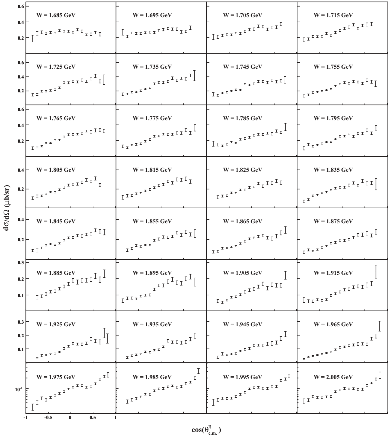
FIG. 5. \frac{d\sigma}{d\Omega}(\mu\text{b/sr}) versus \cos\theta_{c.m.}^{\eta} for the \gamma p \rightarrow p\eta reaction. Note that the vertical axis is linear for W up to 1.965 GeV and logarithmic above that.
