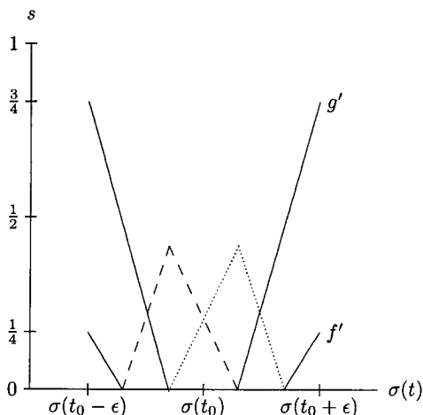
FIGURE 2. Behavior of f' and g' on U . Solid line indicates values in \rho(s) , dotted line indicates values in \gamma(s) , and dashed line indicates values in \lambda(s)
