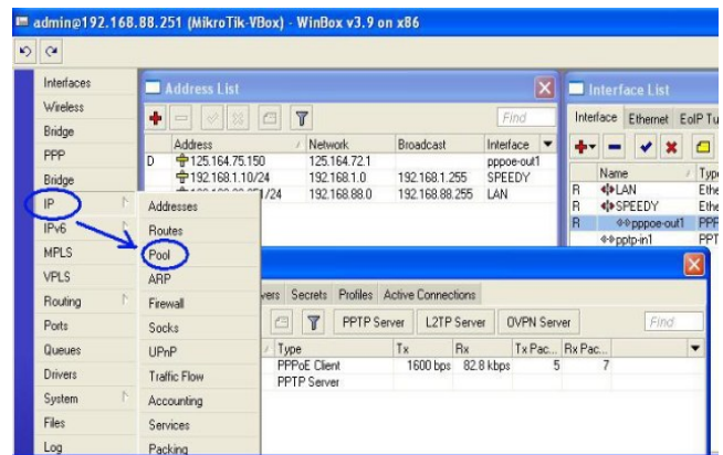
Gambar 9. IP Pool
