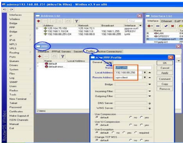
Gambar 12. Profile VPN
