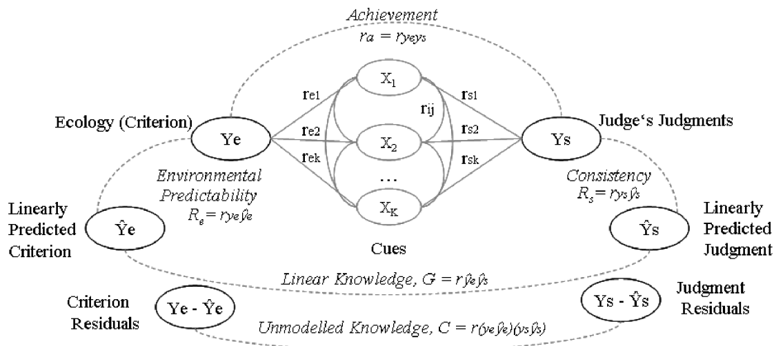
Figure 2. The lens model and the components of the lens model equation.
