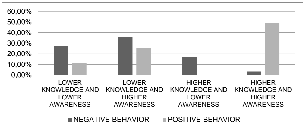
Figure 1. Plot of frequencies across the different categories
