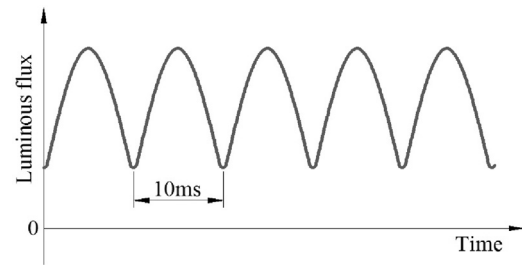
Fig. 2 – Luminous flux of a 3000 K fluorescent tube powered by a voltage at a frequency of 50 Hz (KLC).
