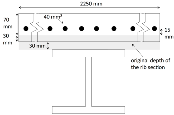
Fig. 2 Composite beam section in Cardington test
