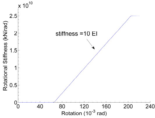
Fig. 4 Semi-rigid connection stiffness of the single-plate connection
