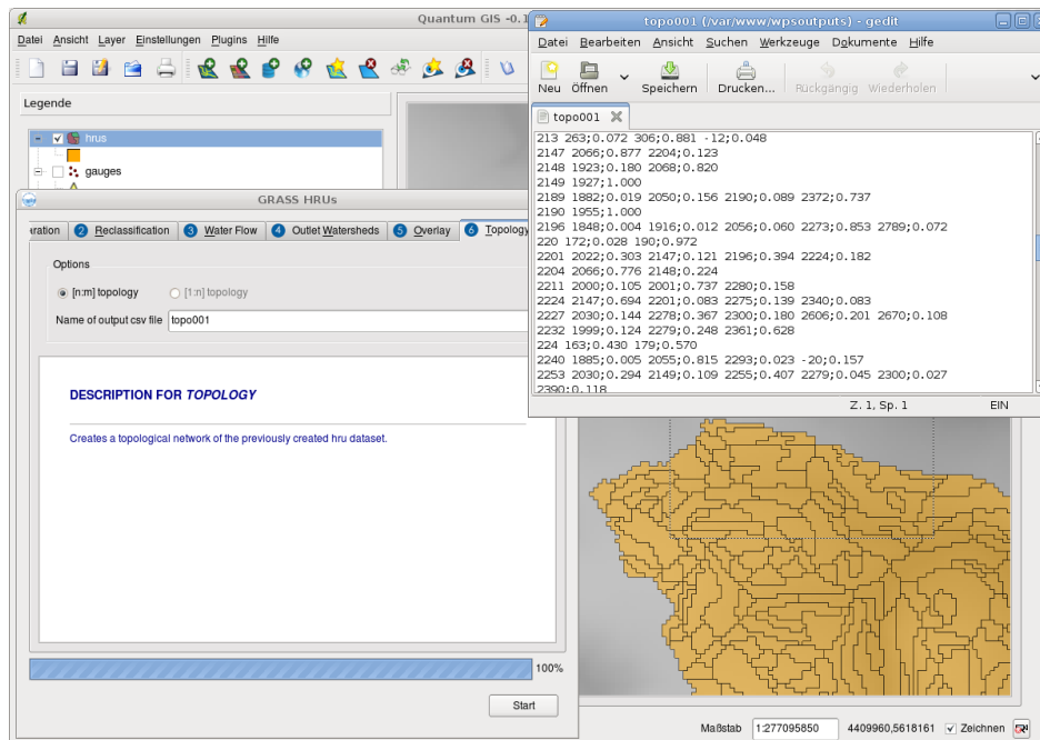
Figure 8: Topology module
