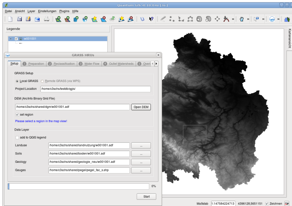
Figure 1: Setup module
