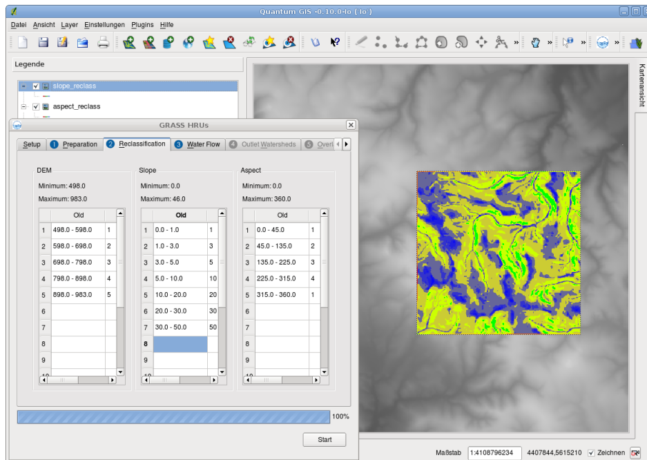
Figure 2: Reclassification module
