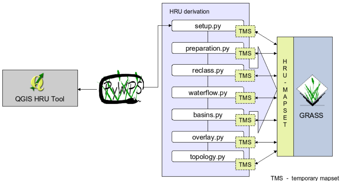
Figure 0: Architecture
