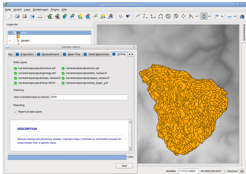
Figure 5: Overlay module
