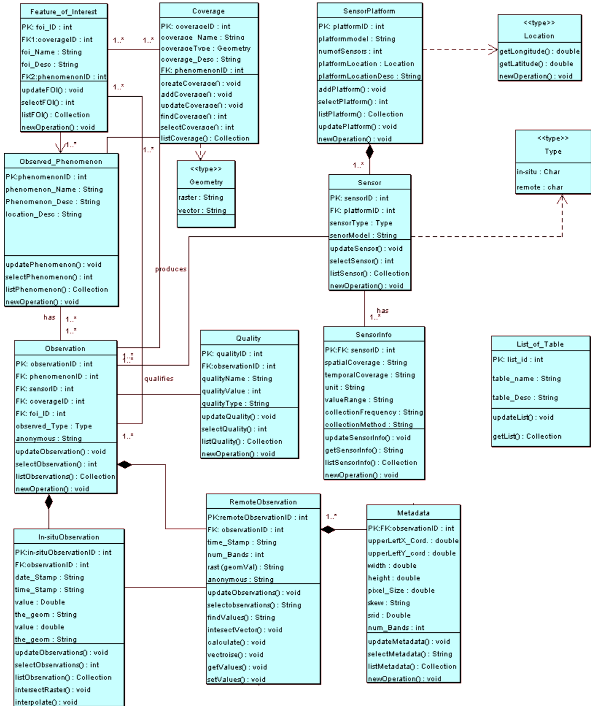
Figure 3: UML Conceptual Schema Model of the Proposed Heterogeneous Sensor Database
