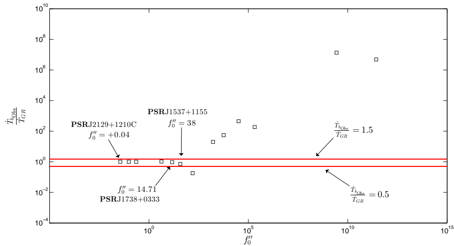
Figure 1: In figure there are shown, for sake of convenience, in logarithmic scale, the absolute values of f_0'' reported in Tab. 1 versus the ratio \frac{\dot{T}_{bObs}}{\dot{T}_{GR}} . We must note that for five binaries the ETGs we are probing is not ruled out 0.04 \leq f_0'' \leq \approx 38 , for those systems the difference between \dot{T}_{GR} and \dot{T}_{bObs} is tiny, indeed we get 0.5 \leq \frac{\dot{T}_{bObs}}{\dot{T}_{GR}} \leq 1.5 . Instead for most of binaries we have f_0'' values that can surely rule out the theory, since taking account of the weak field assumption we obtain 38 \leq f_0'' \leq 4 \times 10^7 . From this last values to the first ones, there is a jump of about four up to five order of magnitude on f_0'' .
