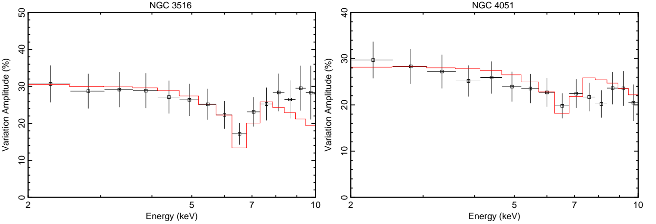
Figure 4: RMS (Root-Mean-Square) spectra for NGC3516 and NGC4051. Black points are calculated from the data, and red-histograms are calculated from the best-fit spectral models for the time-sequence spectra.
