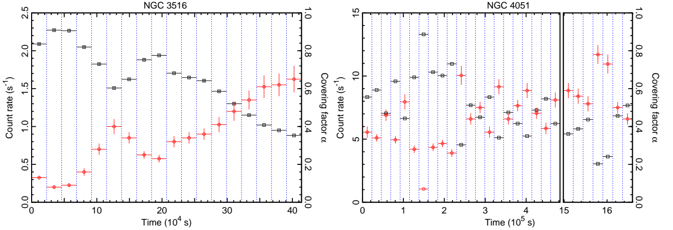
Figure 3: Variations of the observed XIS counting rates (0.2 – 12 keV; black, scale in left) and the partial covering fractions (red, scale in right) for NGC3516 and NGC4051.
