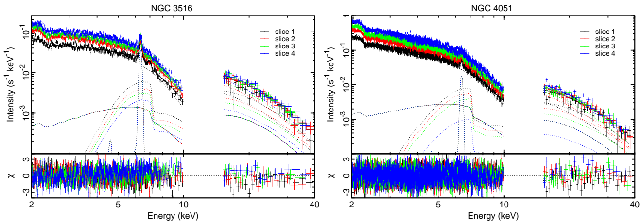
Figure 2: Model fitting results of the intensity-sliced XIS and PIN spectra for NGC3516 and NGC4051. For each observation, the four intensity-sliced spectra are made with approximately equal counts, and the four spectra are fitted simultaneously only varying the partial covering fraction, \alpha . The data and the best-fit power-law model are in the upper panel, while the residuals are in the lower panel.
