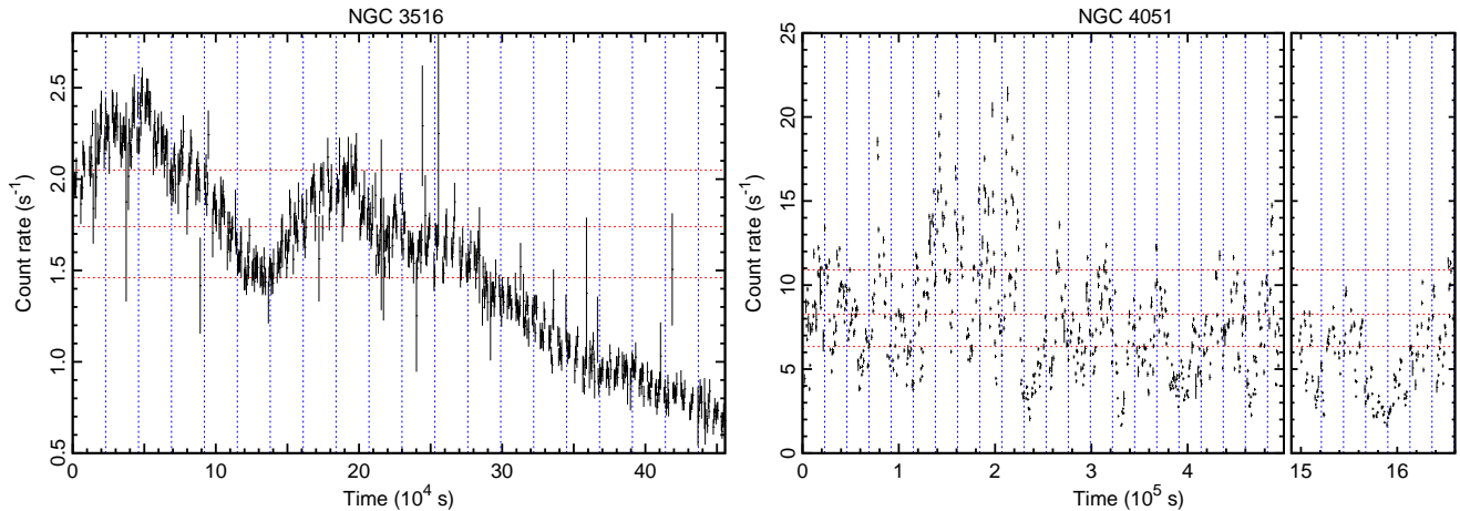
Figure 1: XIS light curves of NGC3516 and NGC4051 in 0.2–12.0 keV. The count rate is binned with 512 s. Horizontal red-dotted lines show the count rate intervals with which the intensity-sliced spectra were made (section 2.2). Vertical blue-dotted lines show the time intervals with which the time-sliced spectra were made (section 2.3).
