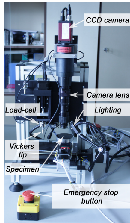
FIGURE 2. Experimental setup.
