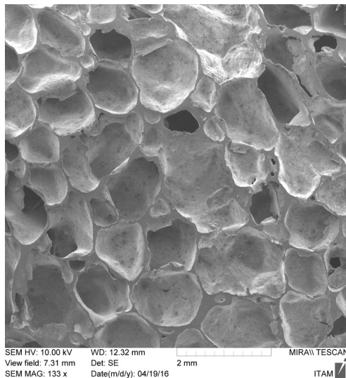
FIGURE 1. Inner structure of aluminium foam obtained by scanning electron microscopy.
