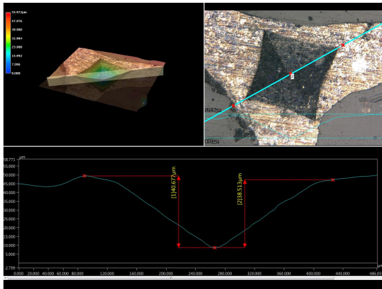
FIGURE 4. Indent surface inspection and indent profile reconstruction equipped by digital microscope.
