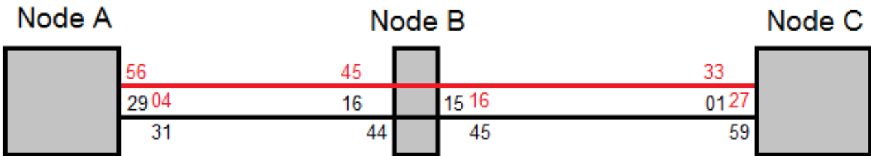
FIGURE 4. Extended timetable descriptors example. Serviced nodes are distinguished with dots of respective colour of the line.
